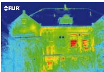
Thermal survey from outside, the red areas represent poor or missing insulation.
