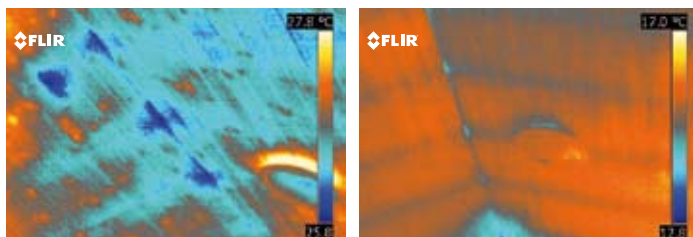
Infrared images taken of the same ceiling. In left image the room temperature has been changed by heating which makes the moisture in the insulation appear clearly.
