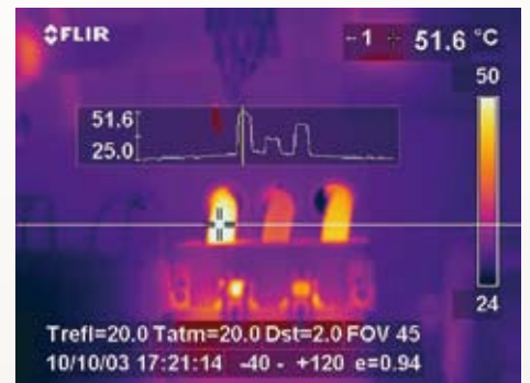
Infrared image of an isolator inspection
