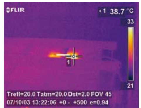
Visual and infrared image of a trip and supply panel.
